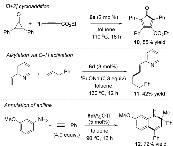
Scheme 5. The application of CAArC-ligated rhodium and gold complexes as active catalysts for the promotion of [3+2] cycloaddition, C–H bond activation, and three-component preparation of 1,2-dihydroquinoline.
