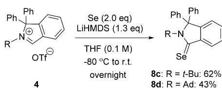
Scheme 3. Synthesis of CAArC-ligated seleno-amides.
