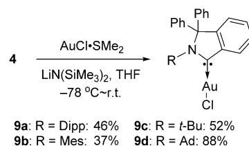
Scheme 4. Synthesis of CAArC-supported gold complexes.
