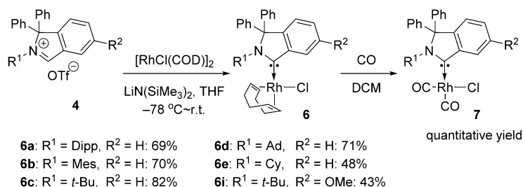
Scheme 2. Synthesis of CAArC-ligated rhodium complexes 6 and 7 .
